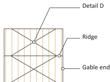
Plan of rafter diagonal bracing layout (narrower fronted detached roof)
